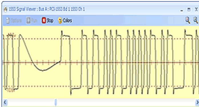
Standard Alta A/D Signal Capture
